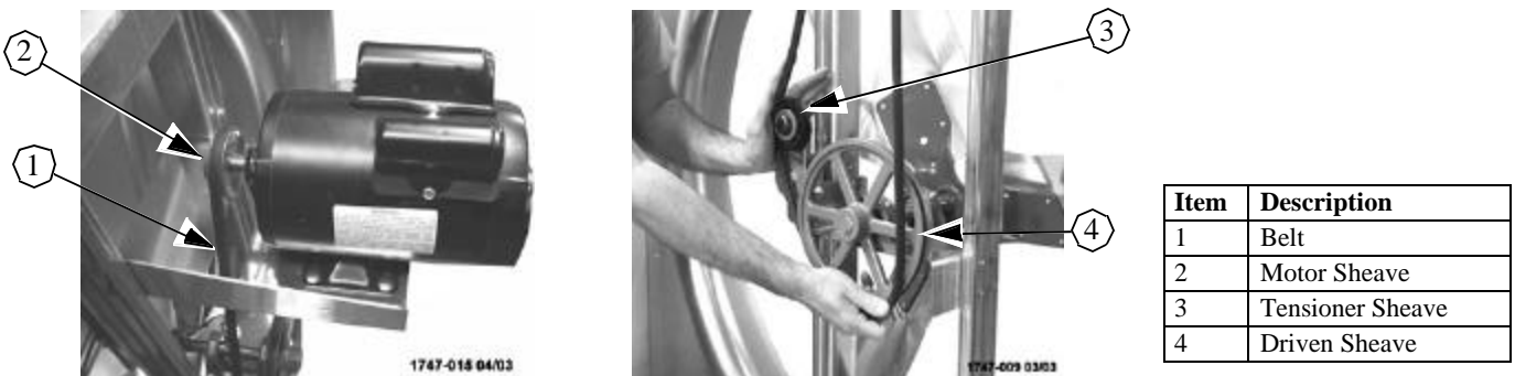
Figure 4. Installing the Belt
