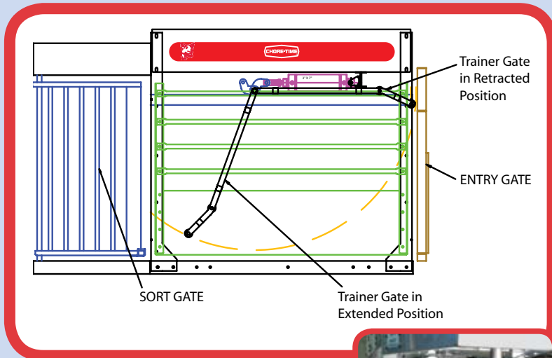
Trainer Gate Assembly (patent pending) helps to keep pigs moving through the scale.
