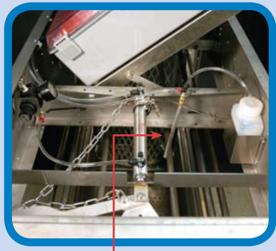
Spray marking option for visual identification of animals.
